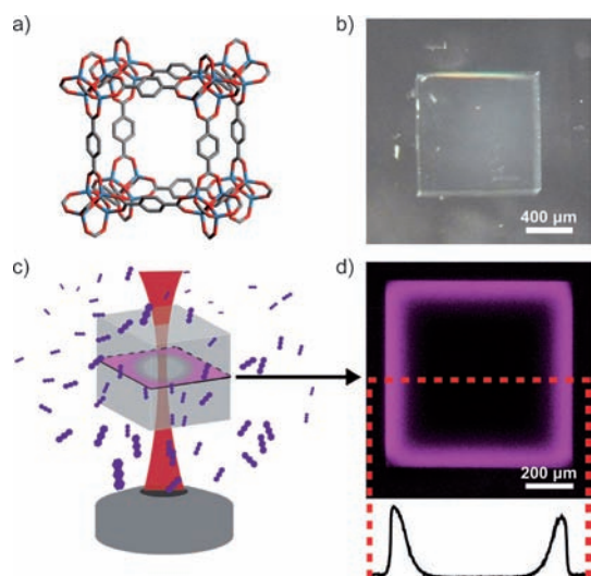
Figure 1. a) A cubic unit cell of a MOF-5 crystal. b) An optical micrograph of a millimeter-sized MOF-5 crystal. c) Experimental setup, in which a single MOF-5 crystal is immersed in a solution of a fluorescent dye (pyronin B) and the three-dimensional intensity/concentration profile is reconstructed using confocal laser scanning microscopy. d) A typical confocal image of an xy section inside of the crystal illustrating the diffusion of the dye (purple). The curve below shows the fluorescence intensity along the horizontal dashed line.
