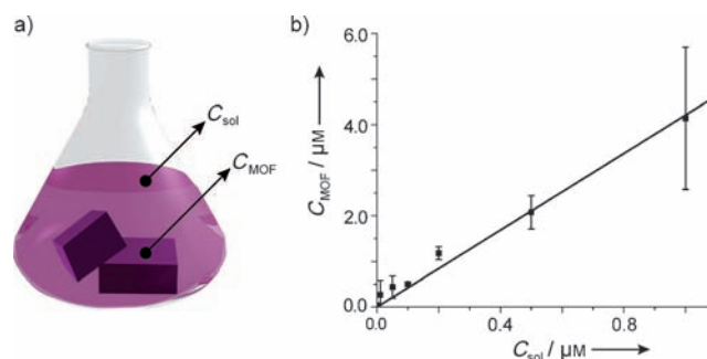
Figure 2. a) Schematic illustration of MOF-5 crystals in a PB solution (not to scale). The equilibrium PB concentration inside MOF-5 crystals ( C_{\text{MOF}} ) and the PB solution concentration ( C_{\text{sol}} ) are indicated. b) C_{\text{MOF}} versus C_{\text{sol}} measured by fluorimetry (see the Experimental Section), which clearly shows that the PB concentration inside the MOF is higher than in solution. Error bars correspond to standard deviations from three independent experiments.
